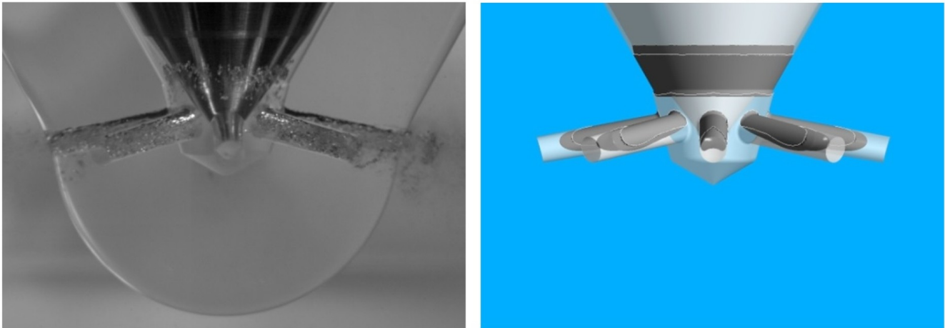
Experimental large scale model and CFD results of the real-size nozzle showing cavitation
